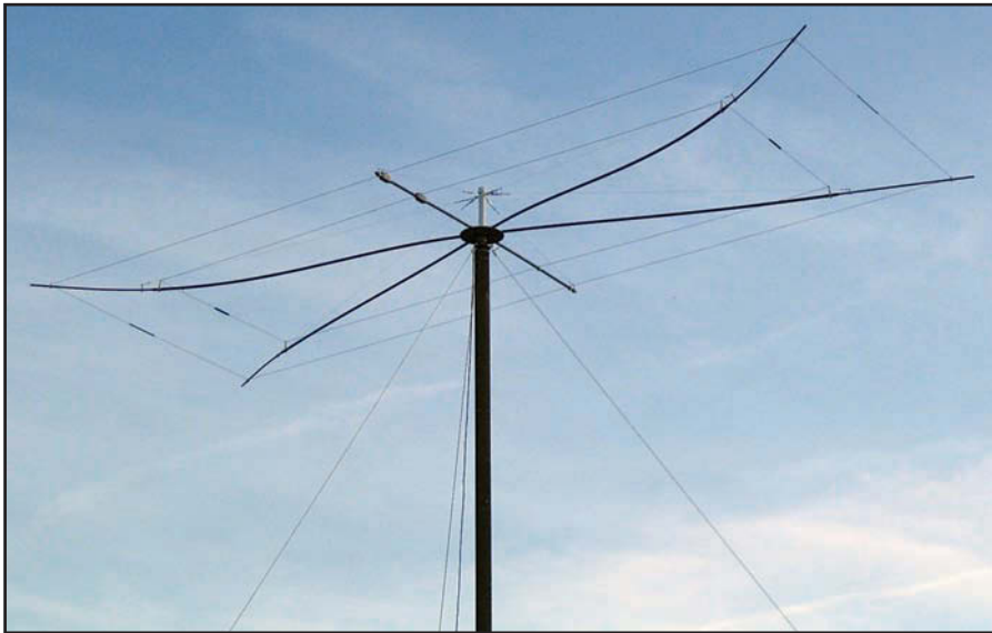
Figure 9—Are the bands open? The completed antenna ready to snag some elusive DX!
